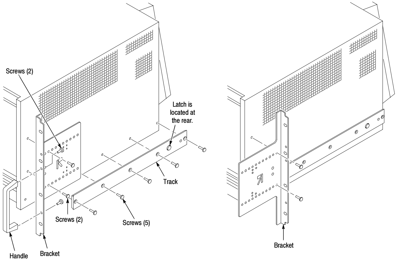
Figure 1: Installing the rackmount kit hardware
