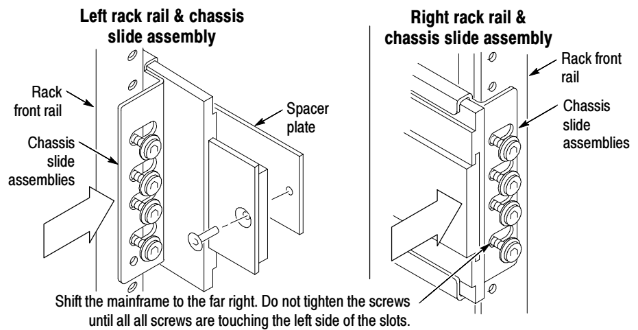
Figure 5: Rackmounting screw positions (front view).
